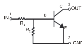
Device Schematics
